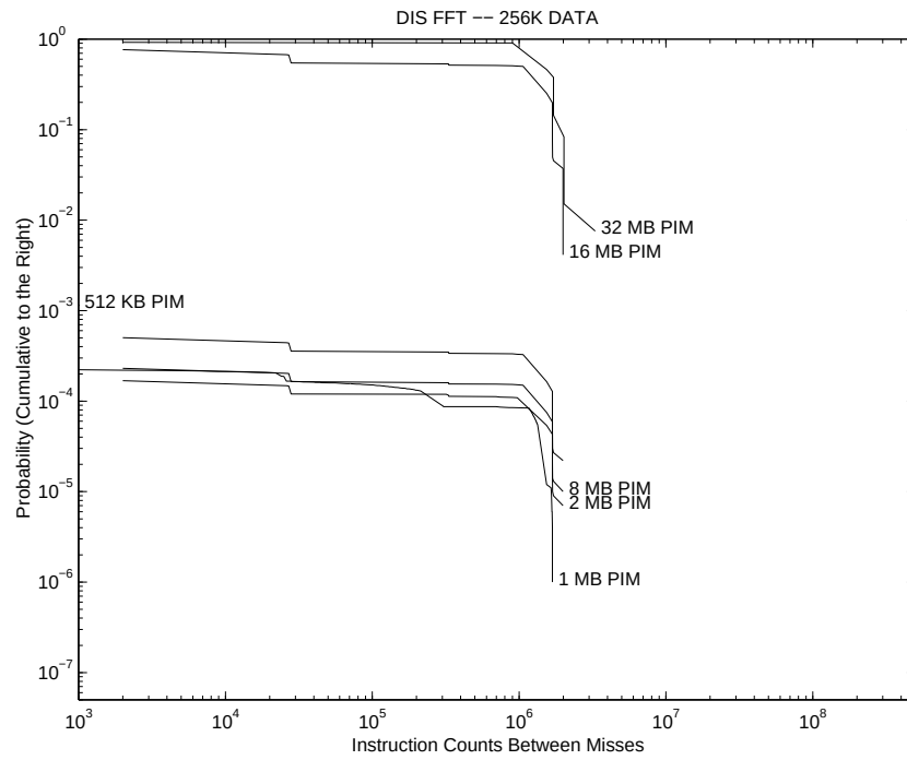
Figure 5.13. DIS FFT 256 KB Page CIPD ( \Psi )
