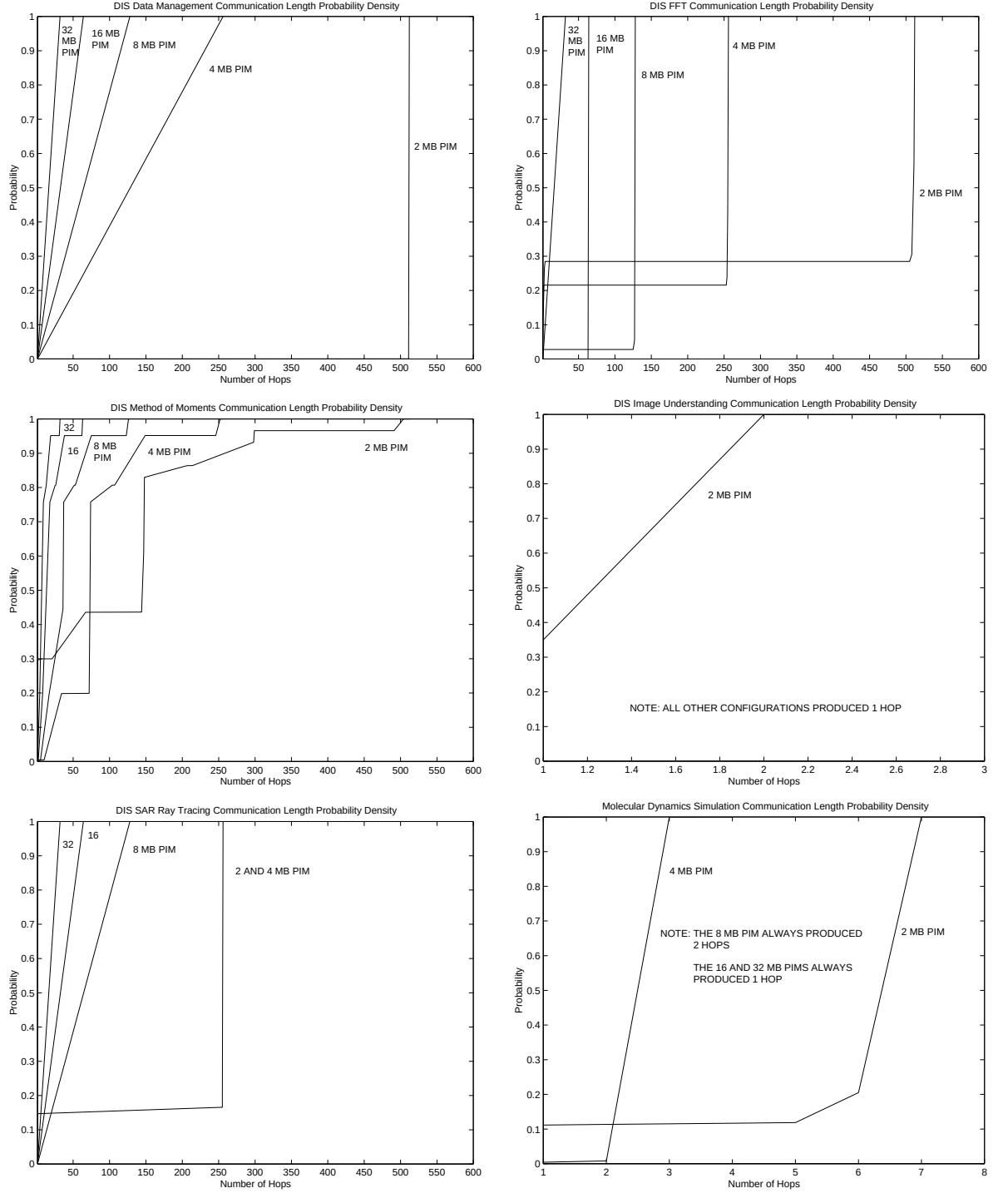
Figure 6.13. Ring CPD (without look-back)
