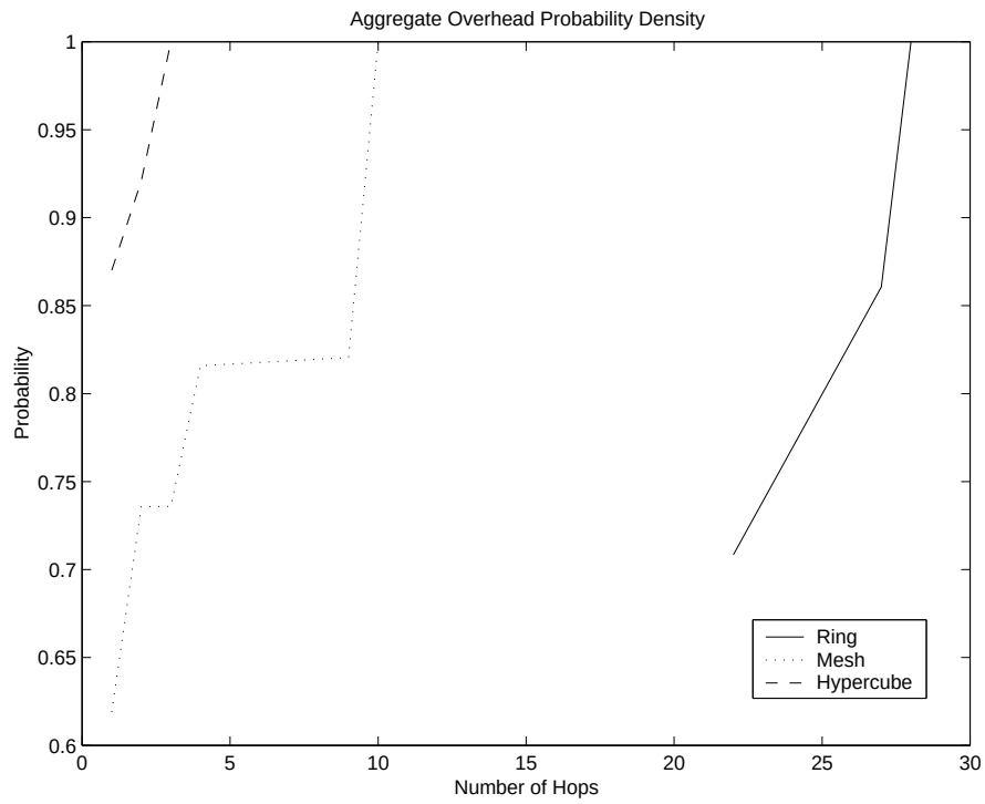
Figure 6.19. Aggregate Overhead
