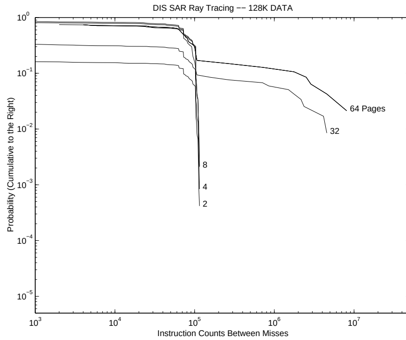
Figure B.62. DIS Ray Tracing 128 KB Page CIPD ( \Psi )
