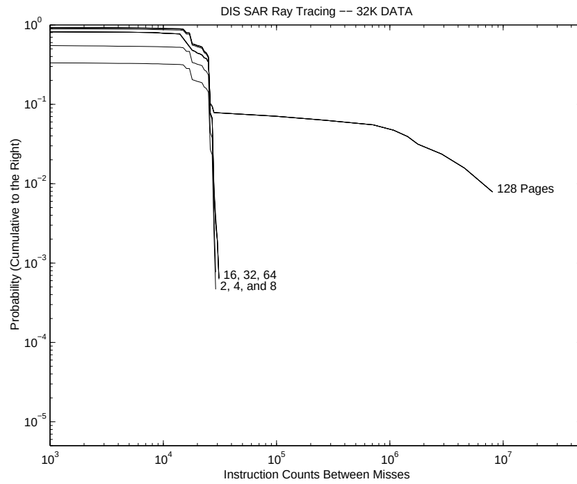
Figure B.60. DIS Ray Tracing 32 KB Page CIPD ( \Psi )
