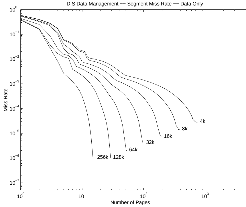
Figure 5.11. DIS Data Management Overall Miss Rate
