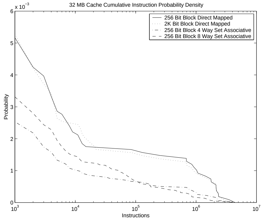
Figure B.70. DIS Ray Tracing 32 MB Data Cache CIPD ( \Psi )
