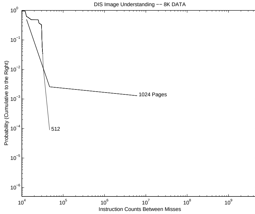
Figure B.44. DIS Image Understanding 8 KB Page CIPD ( \Psi )
