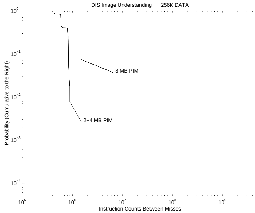
Figure 5.15. DIS Image Understanding 256 KB Page CIPD ( \Psi )
