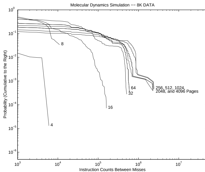
Figure B.72. Molecular Dynamics Simulation 8 KB Page CIPD ( \Psi )
