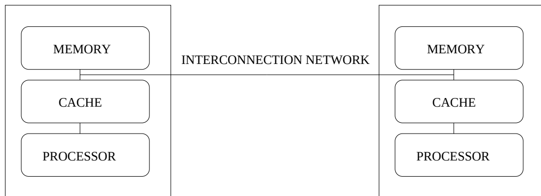
Figure 2.4. A Typical CC-NUMA implementation
