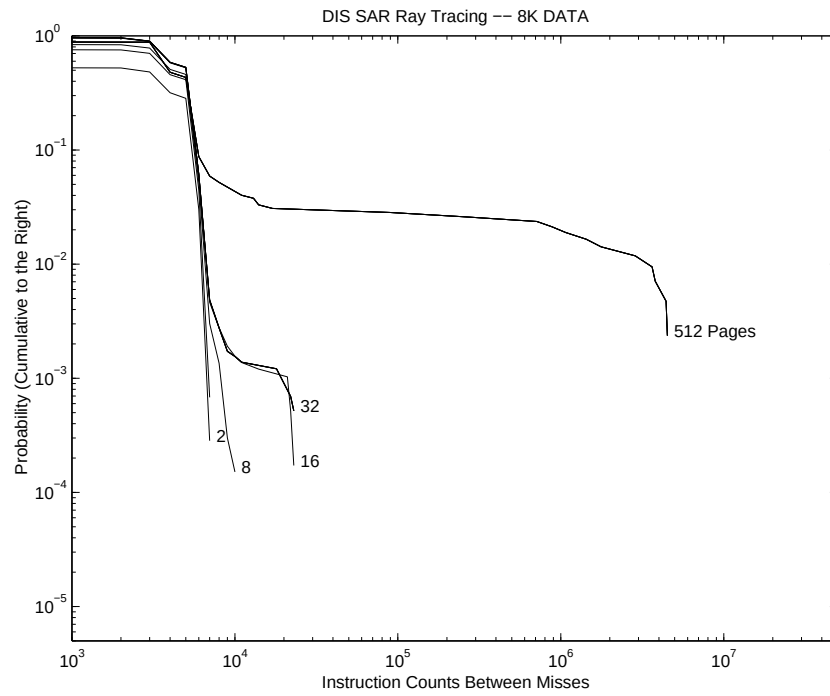
Figure B.58. DIS Ray Tracing 8 KB Page CIPD ( \Psi )
