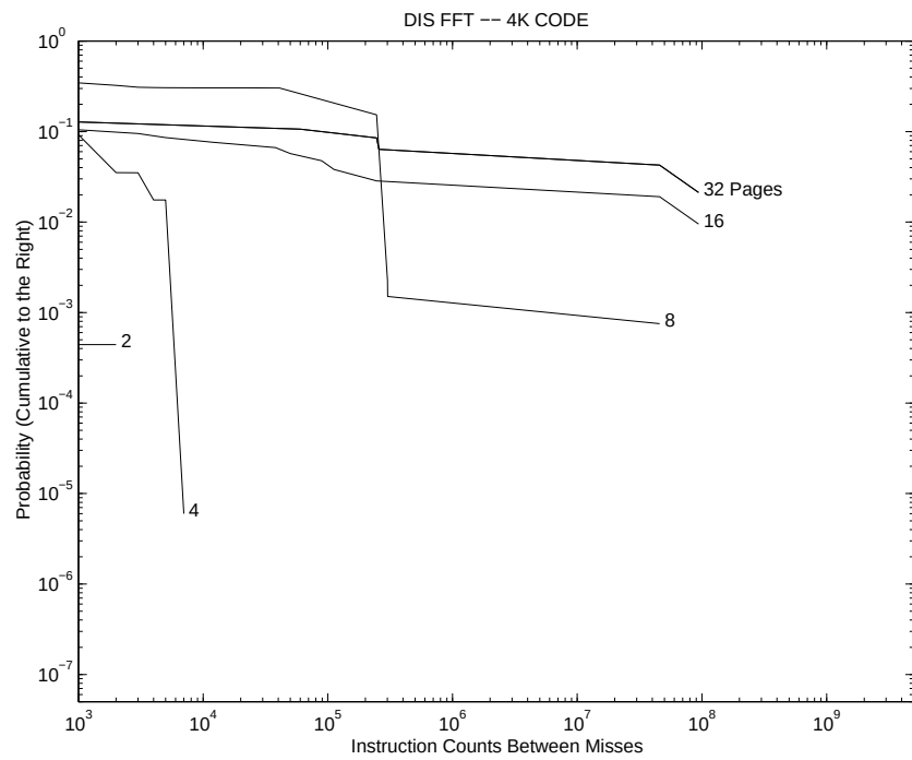
Figure B.22. DIS FFT 4 KB (Code and Stack) KB Page CIPD ( \Psi )
