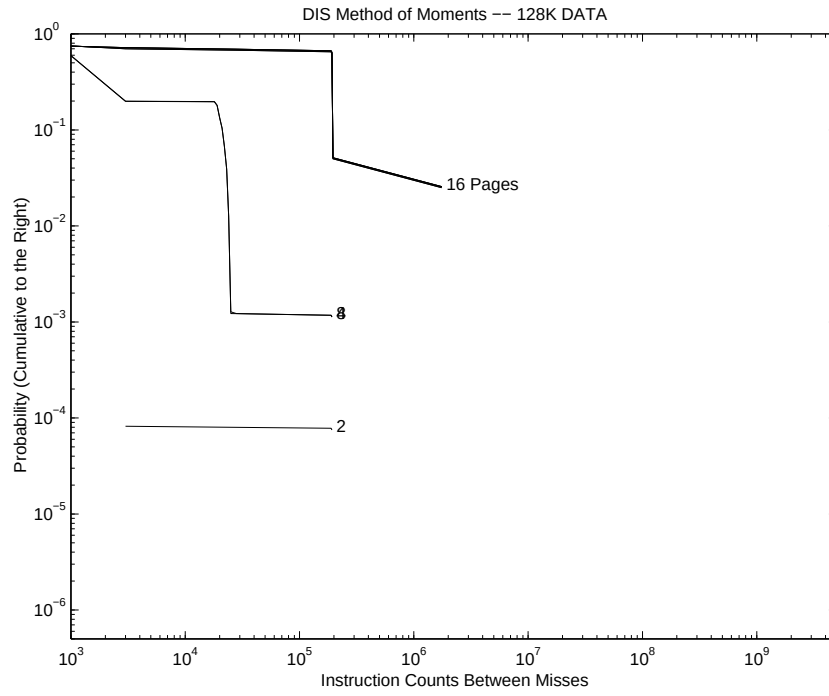
Figure B.34. DIS Method of Moments 128 KB Page CIPD ( \Psi )
