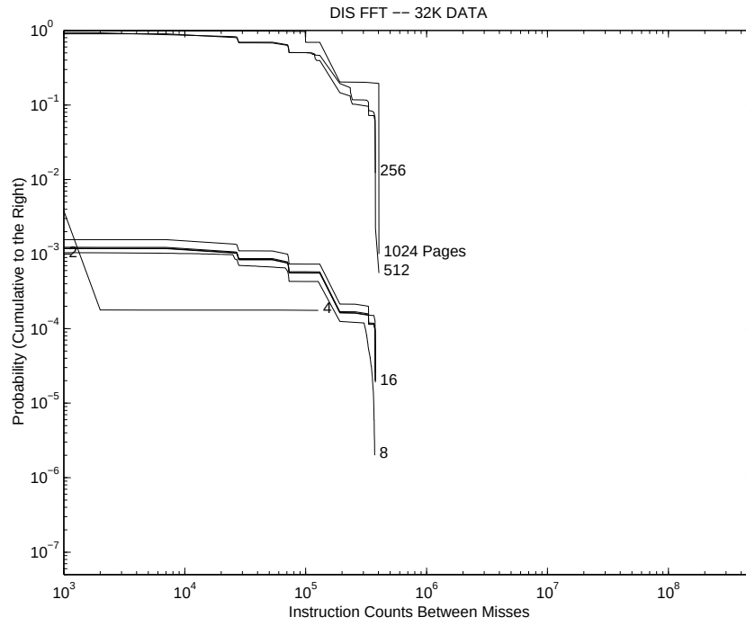
Figure B.18. DIS FFT 32 KB Page CIPD ( \Psi )
