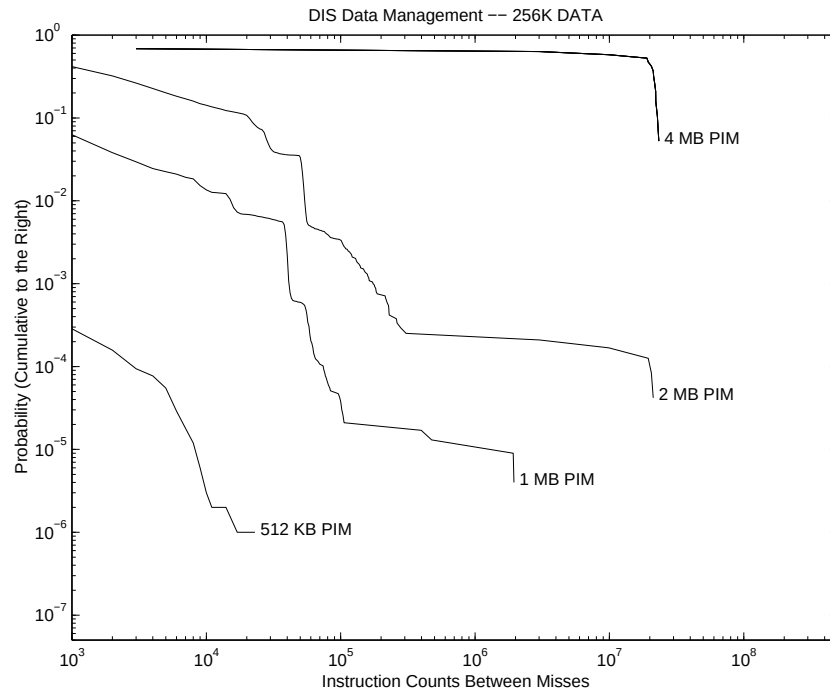
Figure 5.12. DIS Data Management 256 KB Page CIPD ( \Psi )
