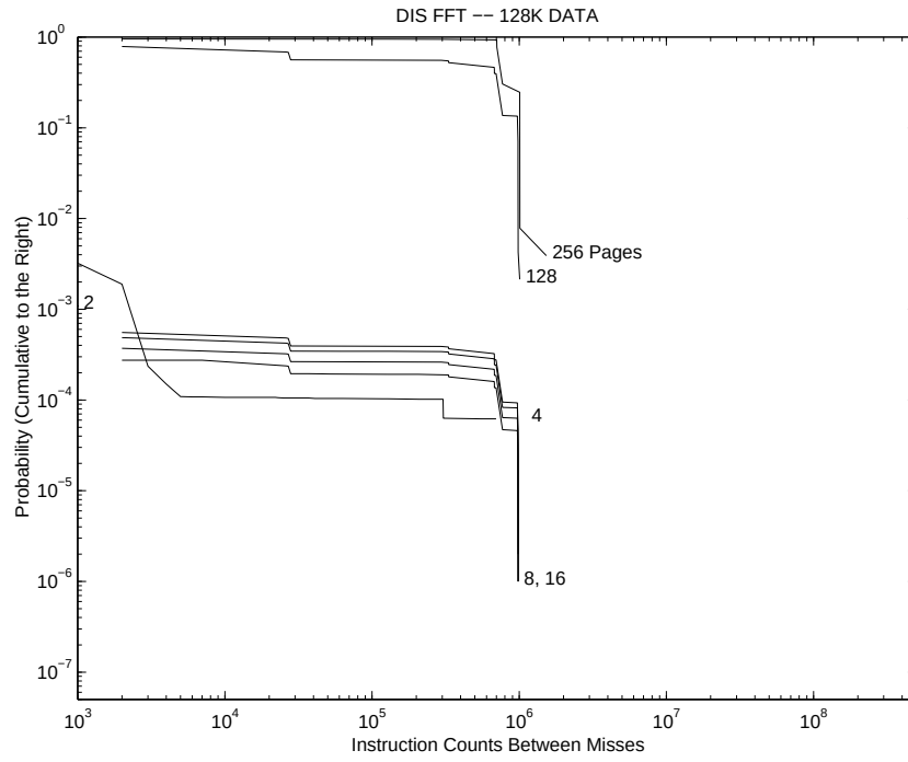
Figure B.20. DIS FFT 128 KB Page CIPD ( \Psi )
