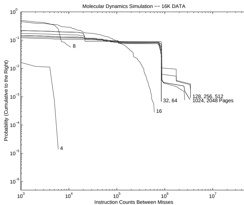
Figure B.73. Molecular Dynamics Simulation 16 KB Page CIPD ( \Psi )
