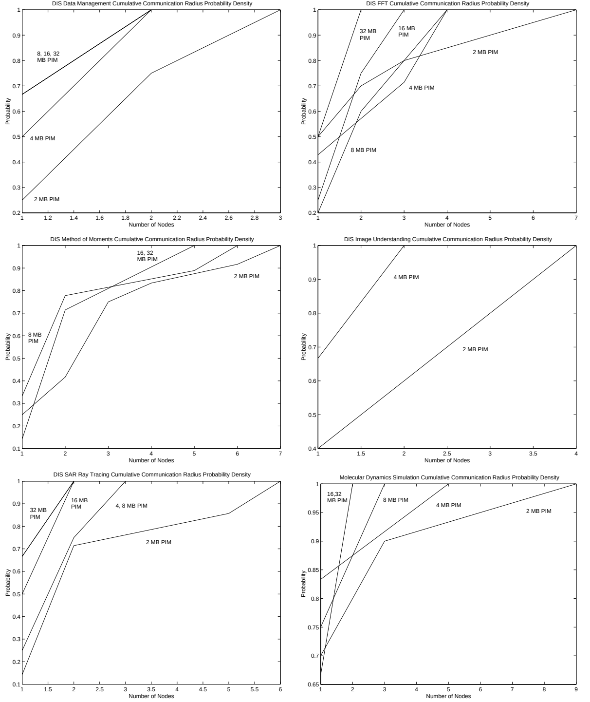
Figure 6.11. Cumulative Communication Radius Probability Density (without look-back)
