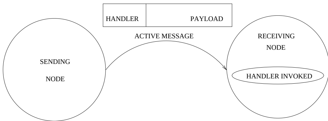
Figure 2.8. Active Messages
